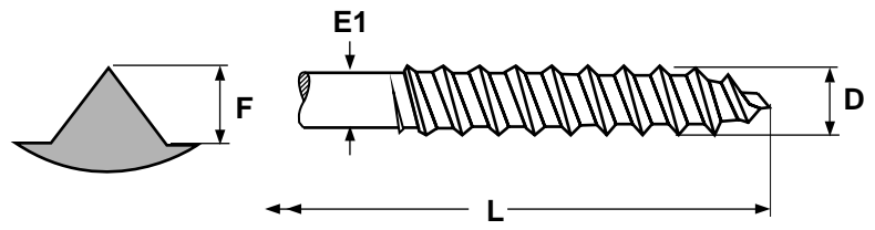
ROLLED THREAD
